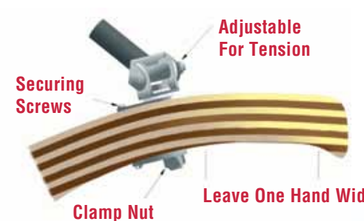
StaFAST™STX & SF
